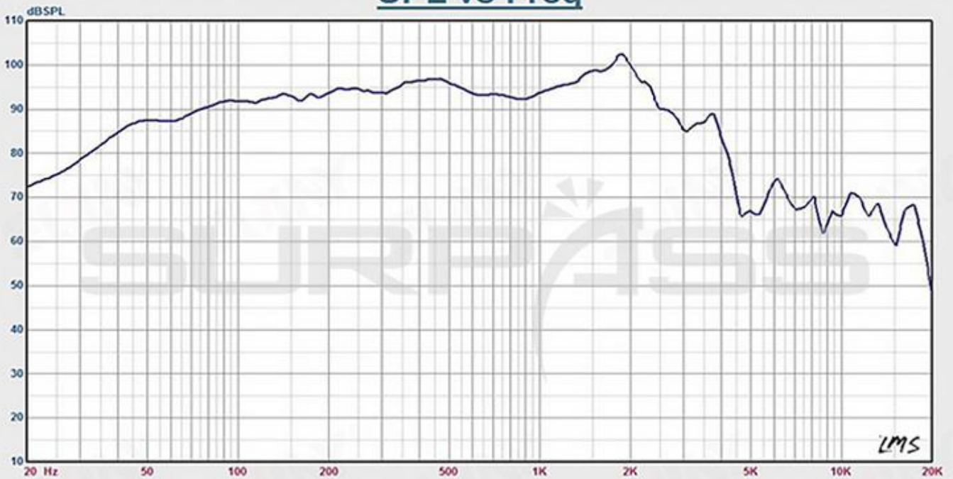
SPL vs Freq
