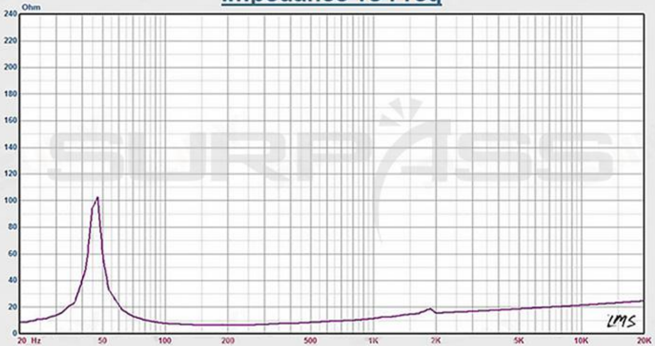
Impedance vs Freq
